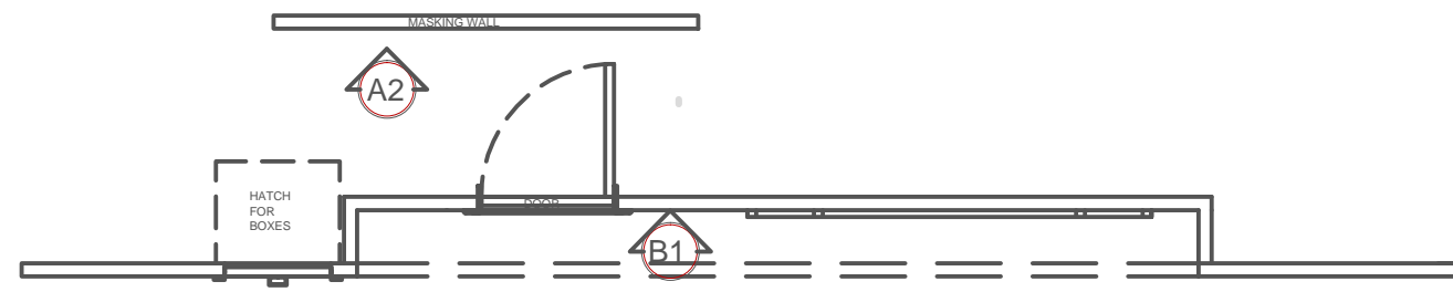
A1 UPSTAGE MAIN WALL: PLAN VIEW
