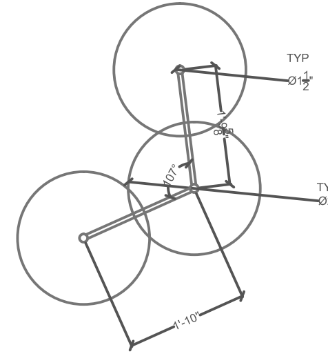
D1 RECEIVING TABLE: PLAN VIEW
